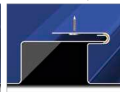
Custom Reveal For 12" Panels up to 3"
